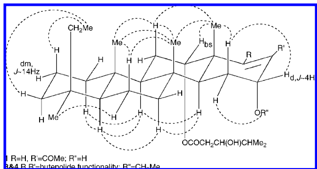
Figure 1. Summary of the significant NOESY correlations (dashed) and J coupling values used to assign the relative stereochemistry of compounds 1 , 3 , and 4 .
